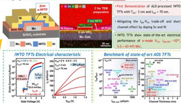
Emerging New Materials for BEOL-devices (Our work at 2025 VLSI Symposium)
