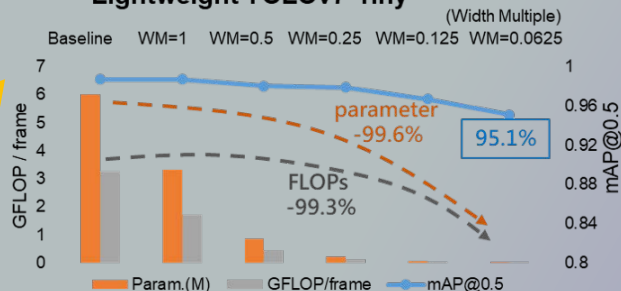
Lightweight YOLOv7-Tiny
